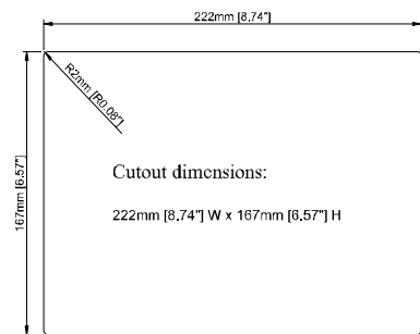
Panel Cutout
